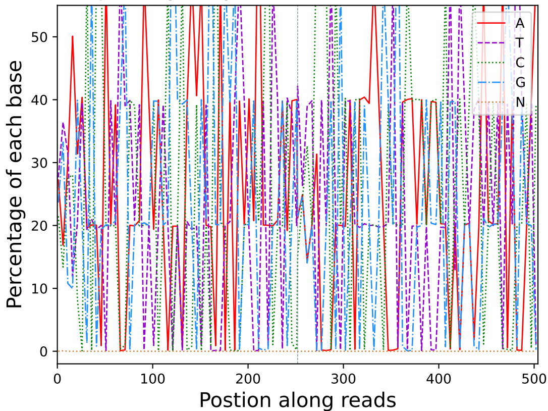
Base percentage along reads (R10610)
